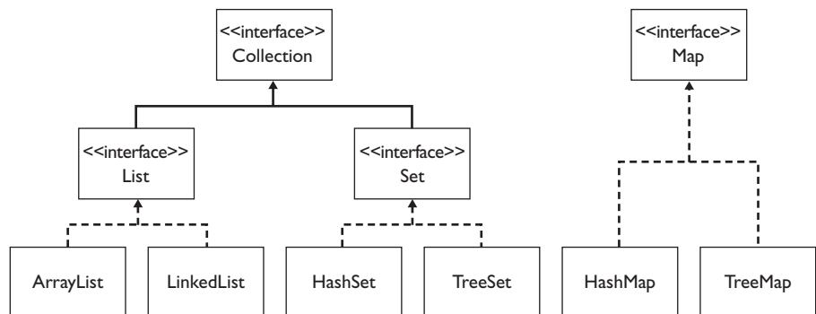
Figure 11.1 An abridged view of the Java Collections Framework
