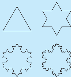
Figure 12.11 Koch snowflake
