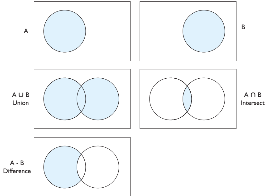
Figure 11.3 Set operation Venn diagrams
