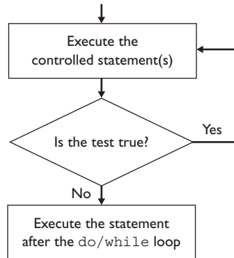
Figure 5.2 Flow of do/while loop
