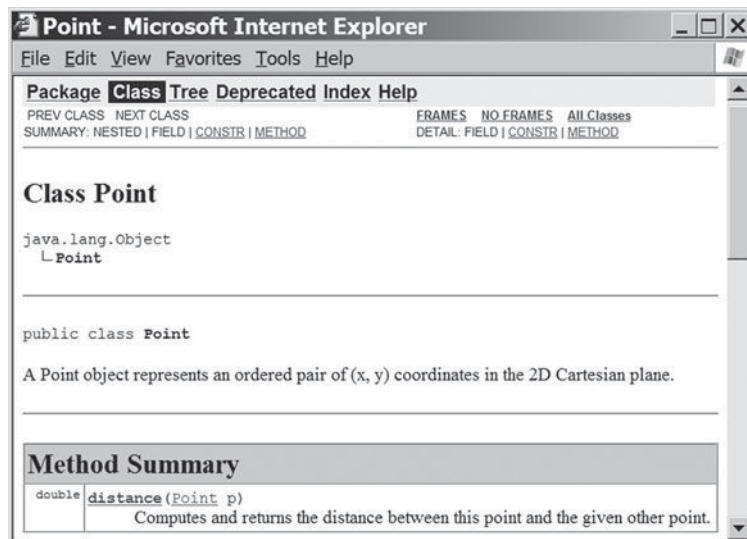
Figure C.2 Generated Javadoc pages for Point class
