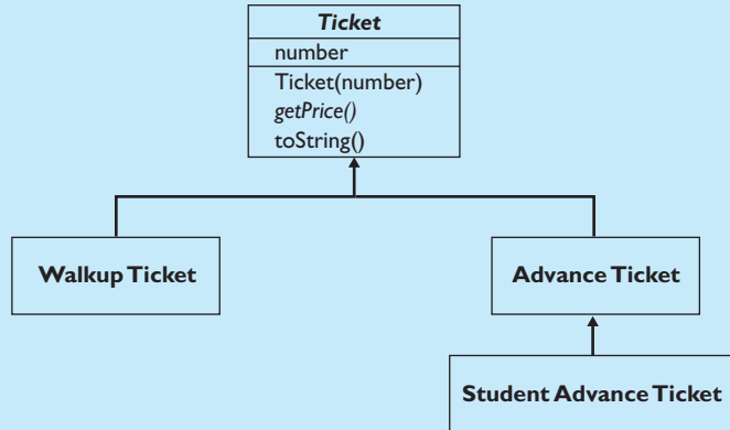
Figure 9.10 Classes of tickets that are available to campus events
