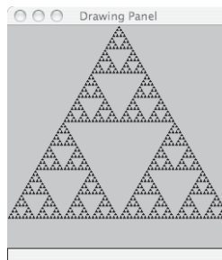
Figure 12.4 Sierpinski triangle, level 7
