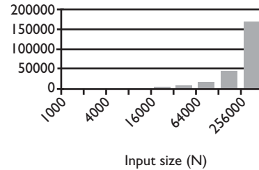
Figure 13.6 Runtimes for selection sort algorithm
