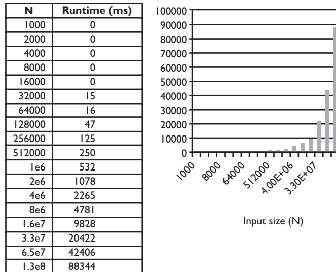
Figure 13.7 Runtimes for merge sort algorithm
