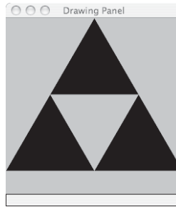
Figure 12.2 Sierpinski triangle, level 2
