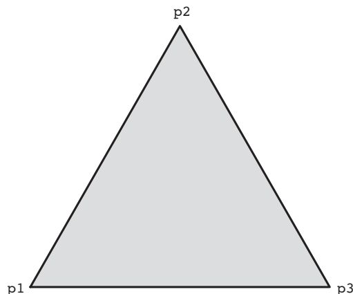
Figure 12.5 Triangle before splitting
