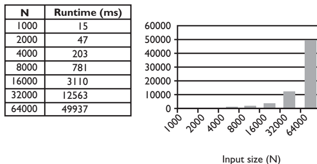
Figure 13.2 Runtimes for first version of range algorithm
