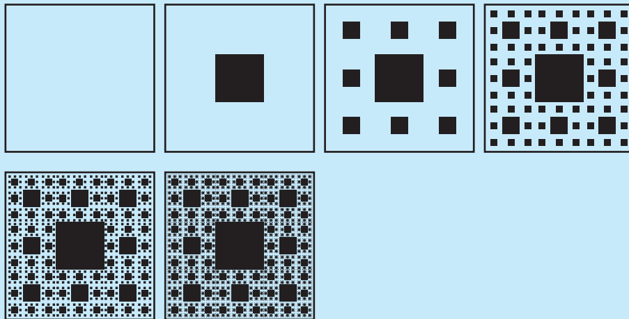
Figure 12.7 Sierpinski carpet
