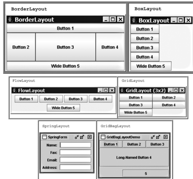
Figure 14.2 Layout managers
