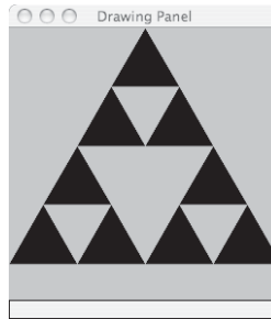
Figure 12.3 Sierpinski triangle, level 3
