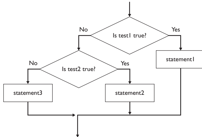
Figure 4.5 Flow of nested ifs ending in else
