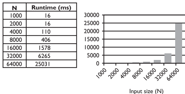
Figure 13.3 Runtimes for second version of range algorithm
