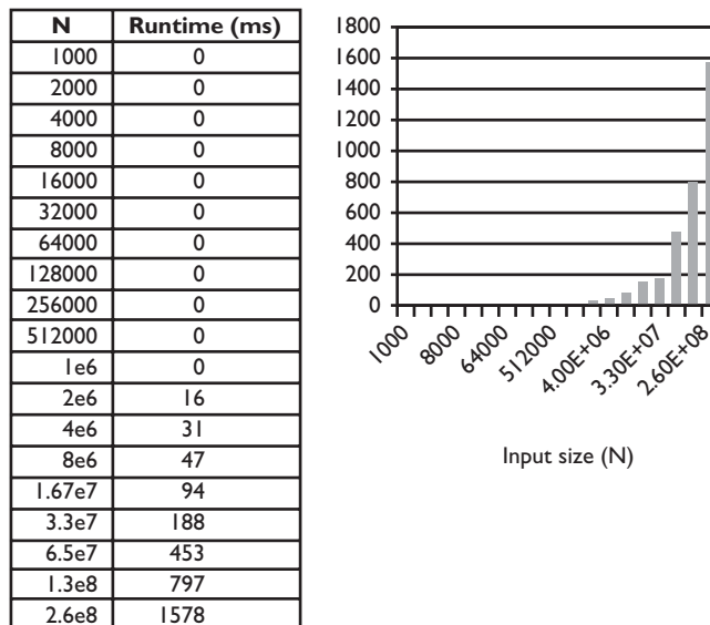
Figure 13.4 Runtimes for third version of range algorithm
