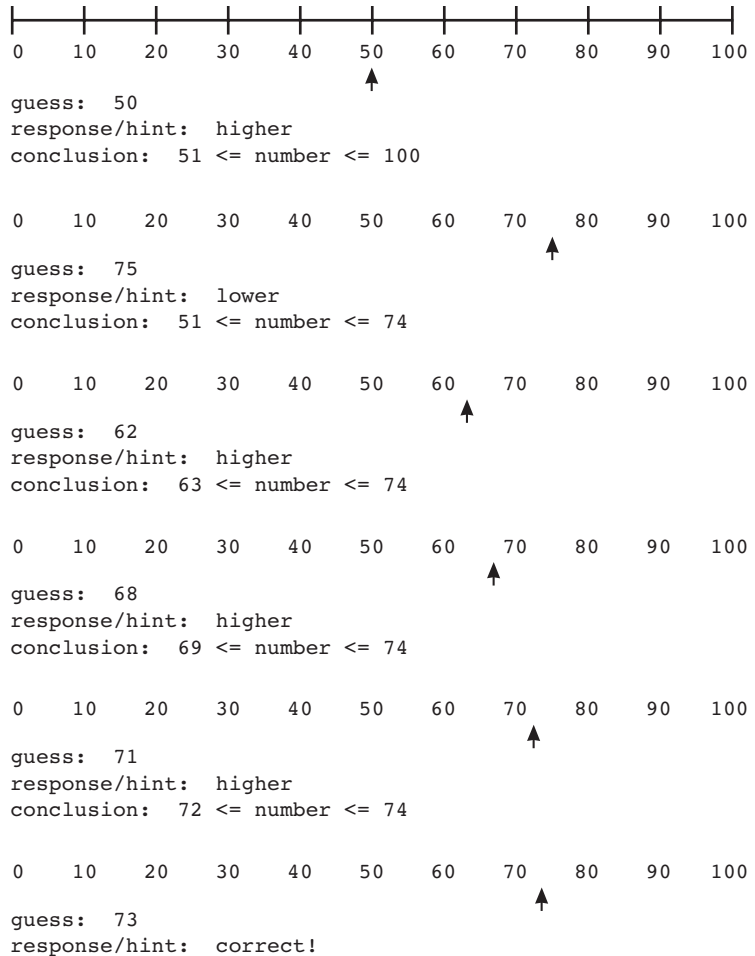
Figure 13.1 Passes of a binary search for a number between 1 and 100
