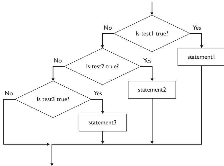
Figure 4.4 Flow of nested ifs ending in test
